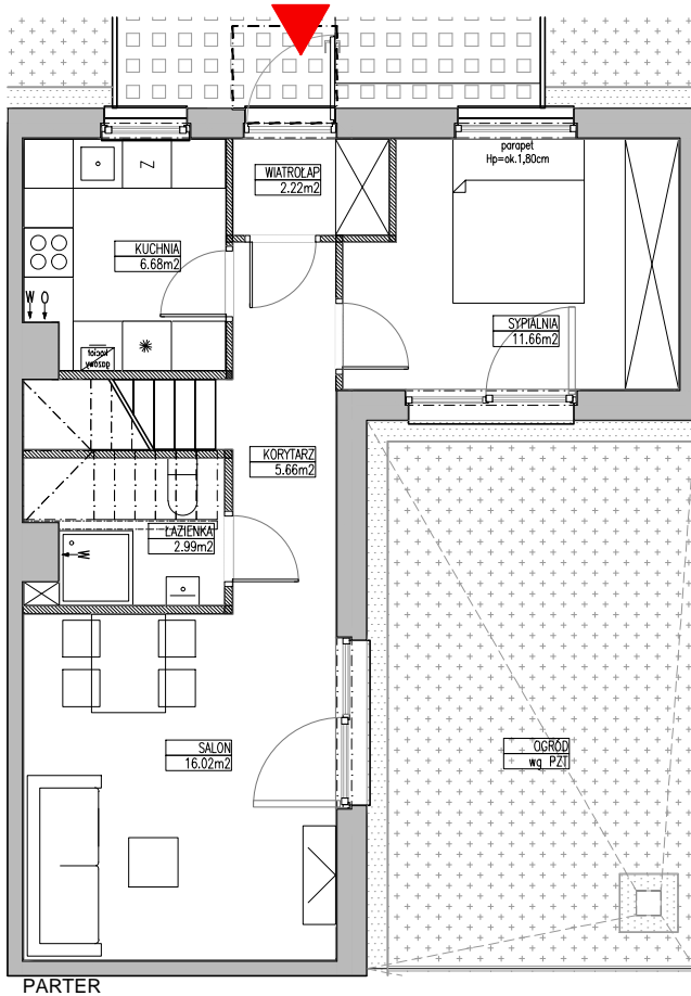
PARTER
